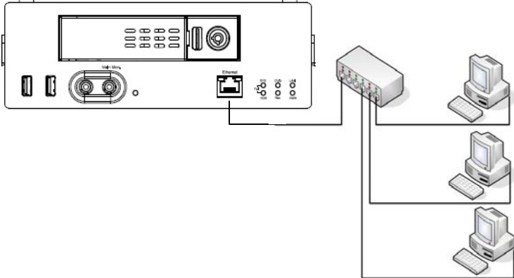
Figure 1-4 Network Connection through Patch Cable
